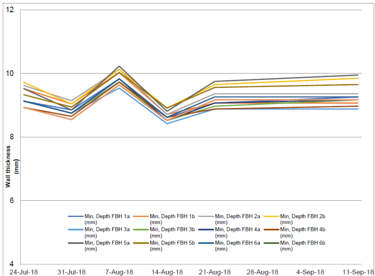
Figure 3: Minimum depth found over time; TFM scan
