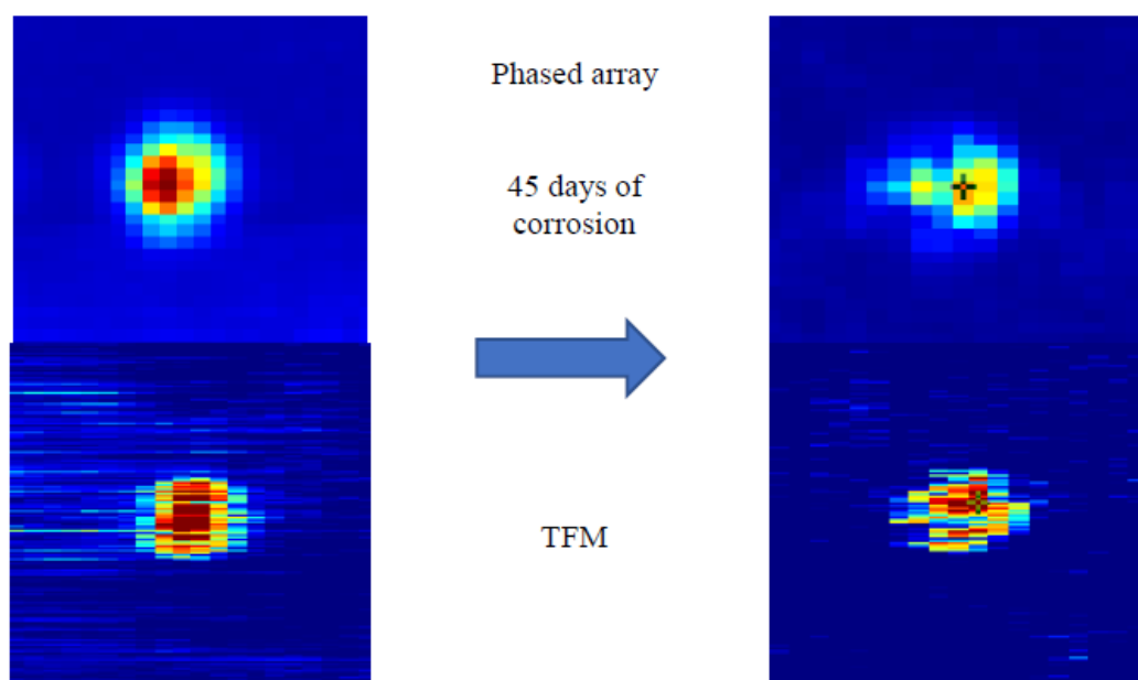
Figure 6: Phased array C-scan and TFM C-scan comparison
